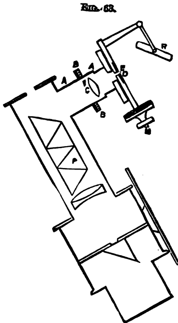
Bright-line Spectro-Micrometer.
